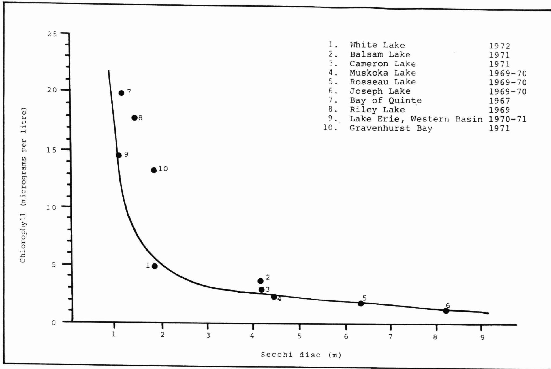
Figure 2: The relationship between chlorophyll a and Secchi disc for White Lake and for a number of other well known recreational lakes in the province. All data are yearly means.
